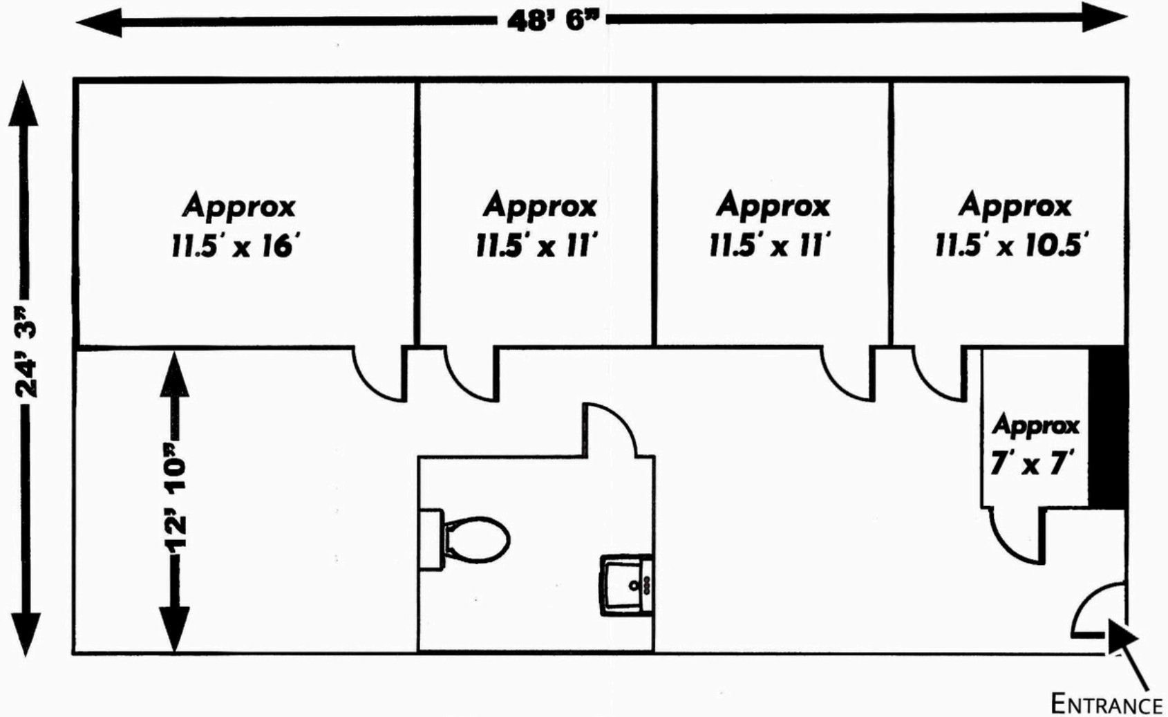
FLOOR PLAN
